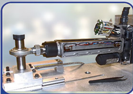
UH-60 Stabilator Linear Actuator Repair & Overhaul
